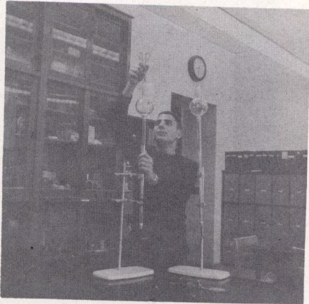
Steve: Adsorption by finely divided or coarsely divided charcoal.
